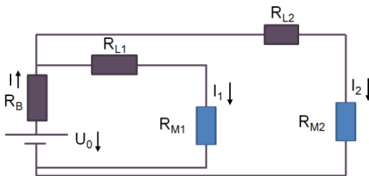
Figure 6.2: Configuration as parallel starters
