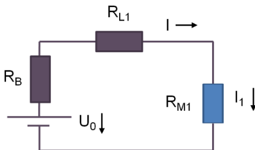
Figure 6.1: Configuration as single starter
